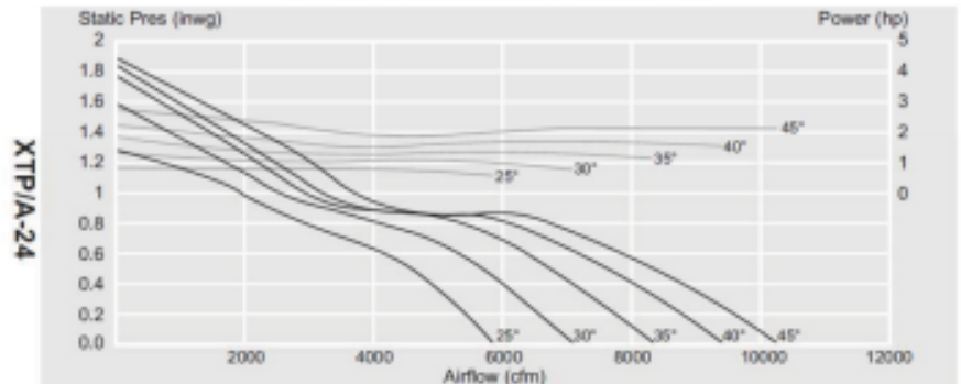
PERFORMANCE CURVES
